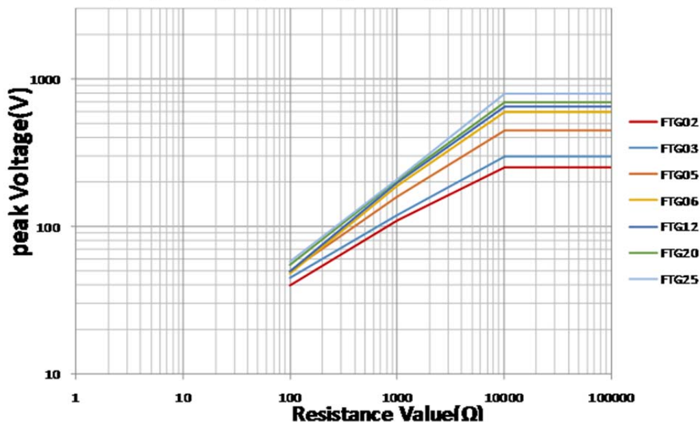
10/70 \mu s Single-pulse high-voltage overload test
